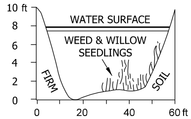
CROSS SECTION 1
