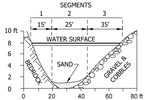
CROSS SECTION 2
